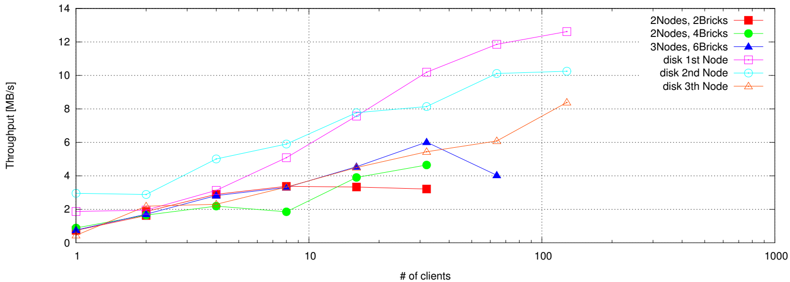
dbench results with and without gluster
